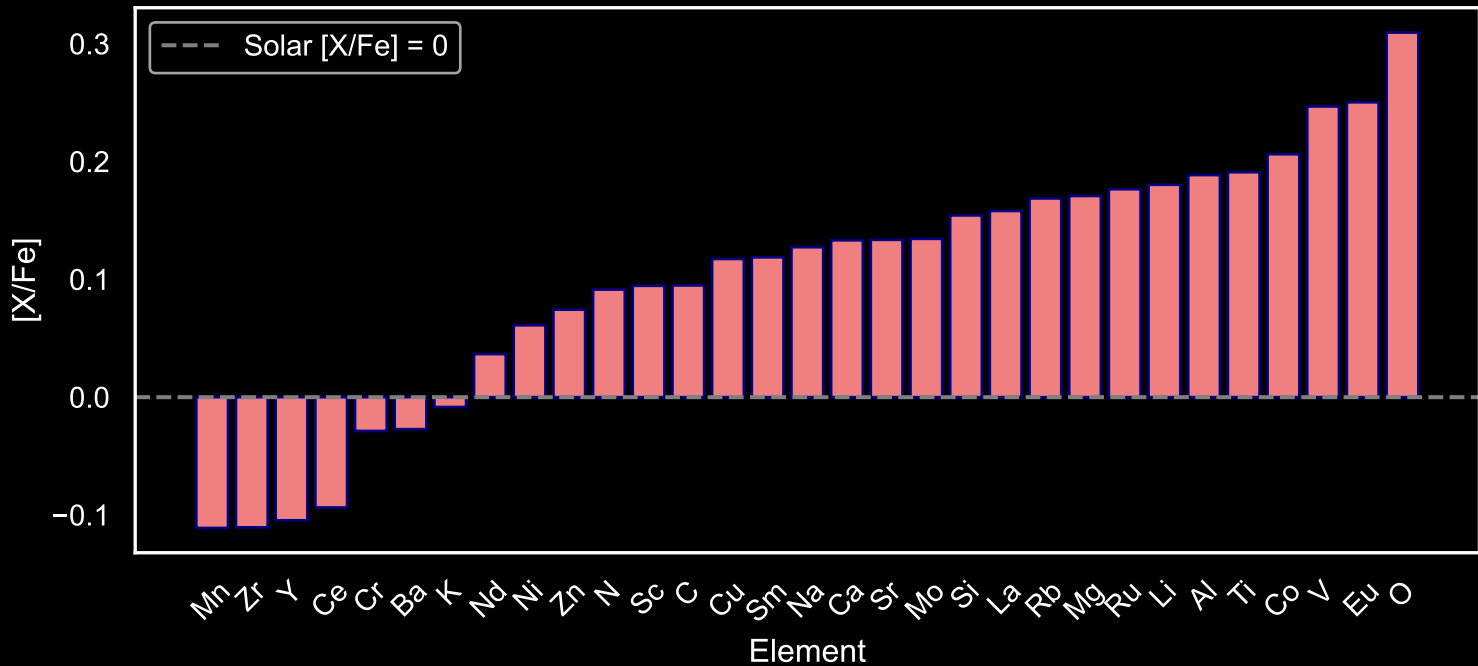
Abundance Pattern for GALAH Red Giants: Star Field [1] (N=42)
