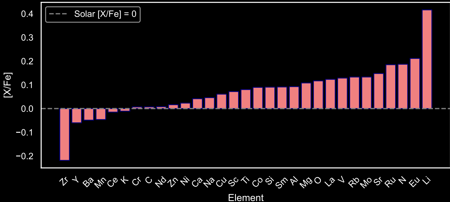
Abundance Pattern for GALAH Star Field [1] (N=222)
