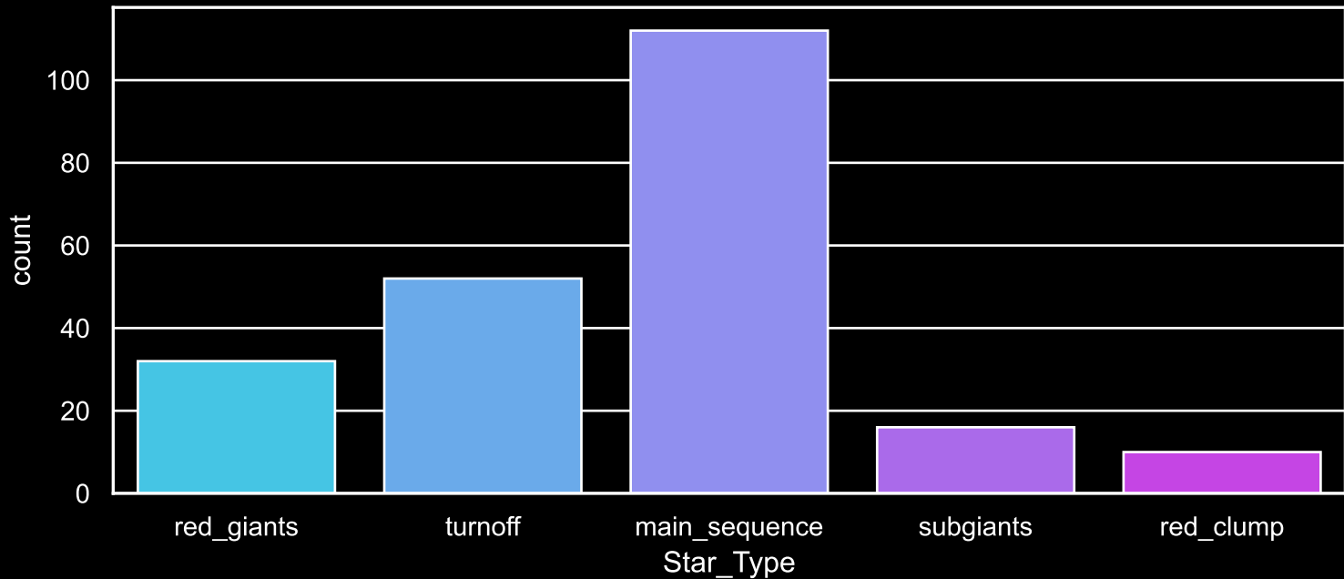
Field [1] Count plot of Star Type
