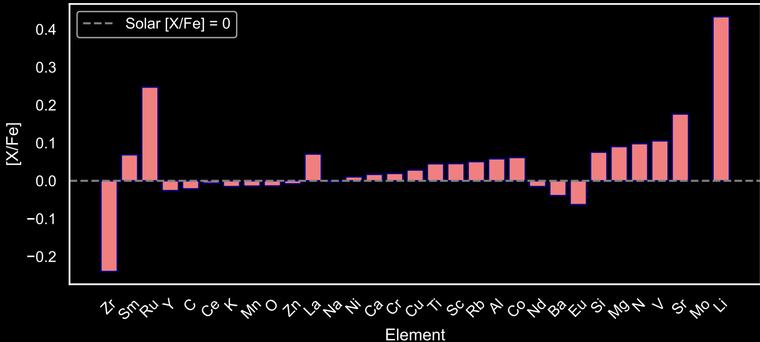
Abundance Pattern for GALAH Main Sequence Stars: Star Field [1] (N=112)
