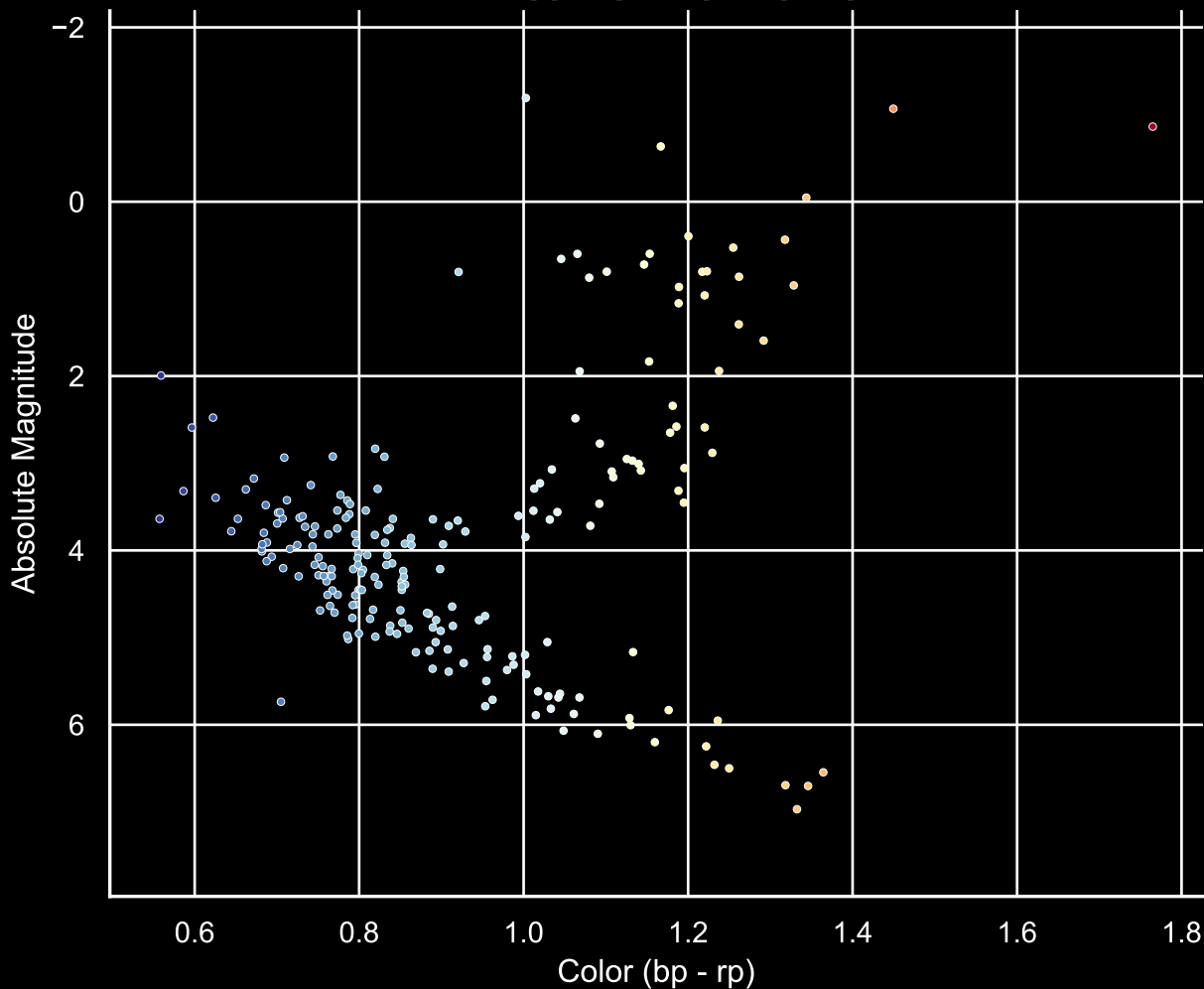
GALAH Hertzprung-Russel Diagram Field [1] Ra [325.33] Dec [-38.9]
